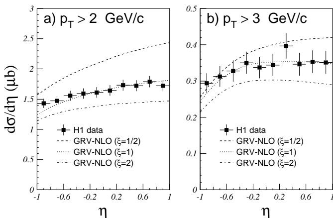
Fig. 4a,b. The differential \gamma p cross-section d\sigma/d\eta for inclusive production of the high p_T charged particles (full squares) in comparison with NLO QCD calculations [36], with different values of the scale, taken as \mu = \xi p_T^2 . The error bars denote the statistical and systematic errors added in quadrature. An overall uncertainty of 5% from the luminosity measurement and electron tagger acceptance is not included
