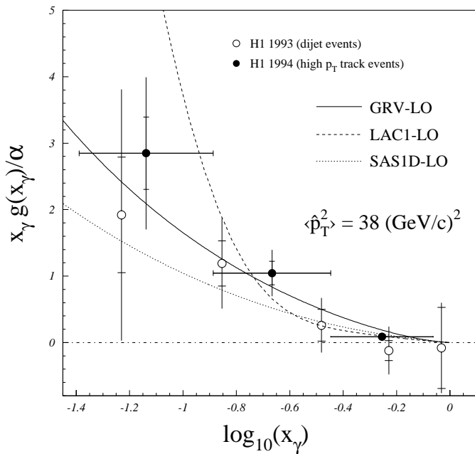
Fig. 7. The LO gluon distribution in the photon from charged tracks (full circles; \langle p_T \rangle^2 = 38 \text{ GeV}^2/c^2 ) and jets (open circles; \langle p_T \rangle^2 = 75 \text{ GeV}^2/c^2 ). The inner error bars are statistical, the full bars are the statistical and systematic errors added in quadrature. An overall uncertainty of 5% from the luminosity measurement and the electron tagger acceptance is not included in the errors. The curves are GRV [21] (full line), SAS1D [22] (dotted line) and LAC1 [23] (dashed line)
