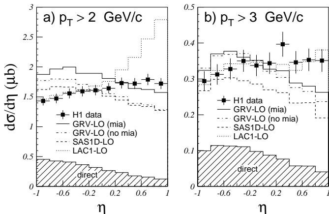
Fig. 3a,b. The differential \gamma p cross-section d\sigma/d\eta for inclusive production of high p_T charged particles (full squares) in comparison with LO QCD calculation by PYTHIA (histograms). The error bars denote the statistical and systematic errors added in quadrature. An overall uncertainty of 5% from the luminosity measurement and electron tagger acceptance is not included. Different lines represent different photon structure function parametrizations: GRV with (full) and without (dash-dotted) multiple interactions, SAS1D (dashed) and LAC1 (dotted). The contributions from the direct photon processes are shown as shaded histograms
