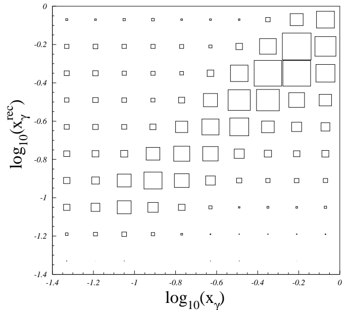
Fig. 5. Correlation between reconstructed and true x_\gamma values using the PYTHIA Monte Carlo with the LAC1 parton densities for the photon
