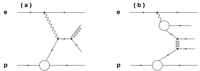
Fig. 1a,b. Examples of diagrams for direct a and resolved b photon processes in ep scattering; in b a gluon has the space-like virtuality of the probe and a quark is resolved in the photon; similarly gluons in the photon can be resolved by quarks and gluons with space-like virtuality
