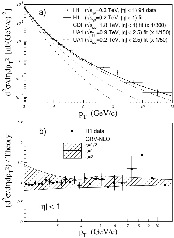
Fig. 2. a The inclusive \gamma p cross-section for charged particles in photoproduction (full squares) measured in the kinematical region |\eta| < 1.0 at an average \sqrt{s_{\gamma p}} \approx 200 GeV. The error bars denote the statistical and systematic errors added in quadrature. An overall uncertainty of 5% from the luminosity measurement and the electron tagger acceptance is not included in the errors. The curves indicate power-law fits, as described in the text, for these data and for the p\bar{p} data from UA1 and CDF as given in [32,33]. b The ratio of data over the NLO QCD calculation with scale \xi p_T^2 for \xi = 1 . The shaded band shows the expected variation of the ratio as \xi changes from 0.5 to 2, illustrating the sensitivity of the QCD calculation to the renormalization and factorization scales (see text)
