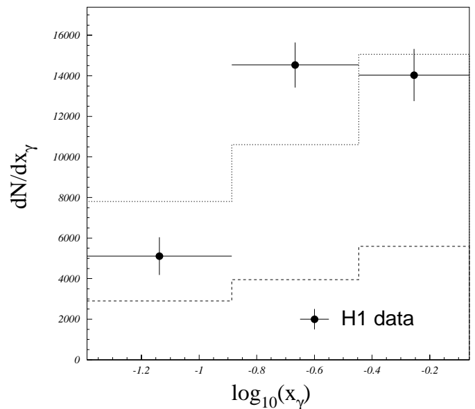
Fig. 6. The x_\gamma distribution in the photon. The errors are statistical only. The curves are full (dotted line) and ‘quark only’ (dashed line) predictions of PYTHIA, using the LAC1 parton distributions of the photon
